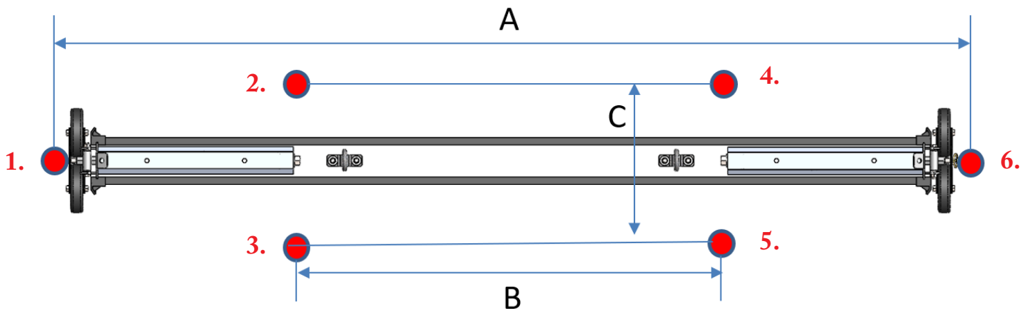
6 Suspension Mounting Point Locations relative to the ISO
